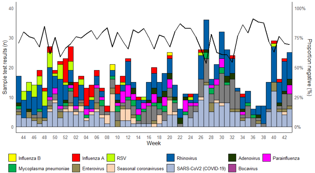
Figure 3.4. Samples submitted for virological testing from ICU patients, by week of sample collection, Week 43, 2023 to Week 43, 2024. The black line indicates the percentage of samples which tested negative for any of the pathogens listed.
