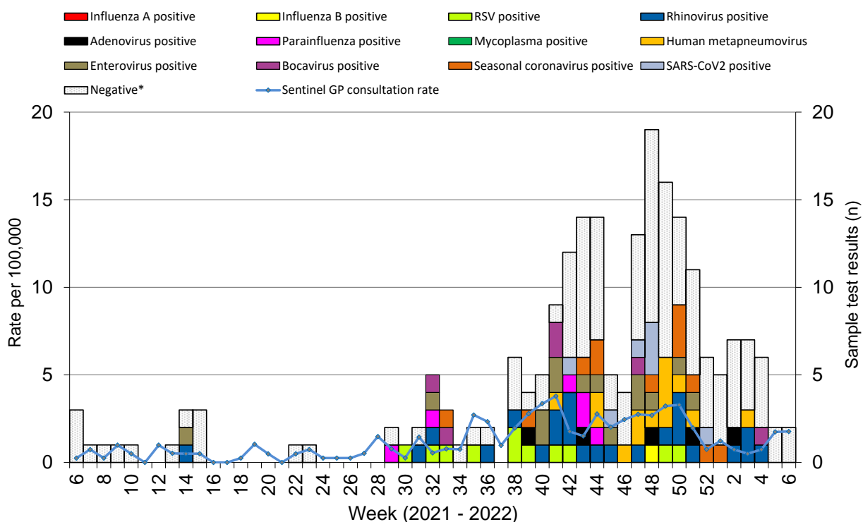
Figure 3. Specimens submitted for virological testing by sentinel GPs as of 13/02/2022, by week of sample collection, week 06 2021 to week 06 2022.
