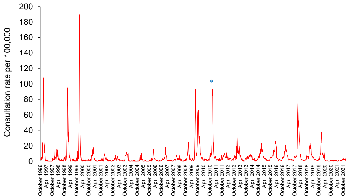
Figure 2. Clinical consultation rate for ILI per 100,000 practice population in Welsh sentinel practices (week 48 1996 – week 06 2022).
