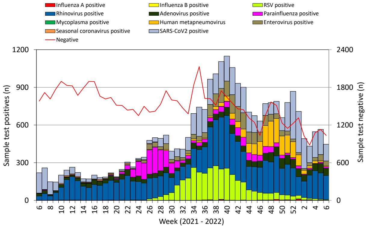
Figure 4. Specimens submitted for virological testing for hospital patients and non-sentinel GPs as of 13/02/2022 by week of sample collection, week 06 2021 to week 06 2022.
