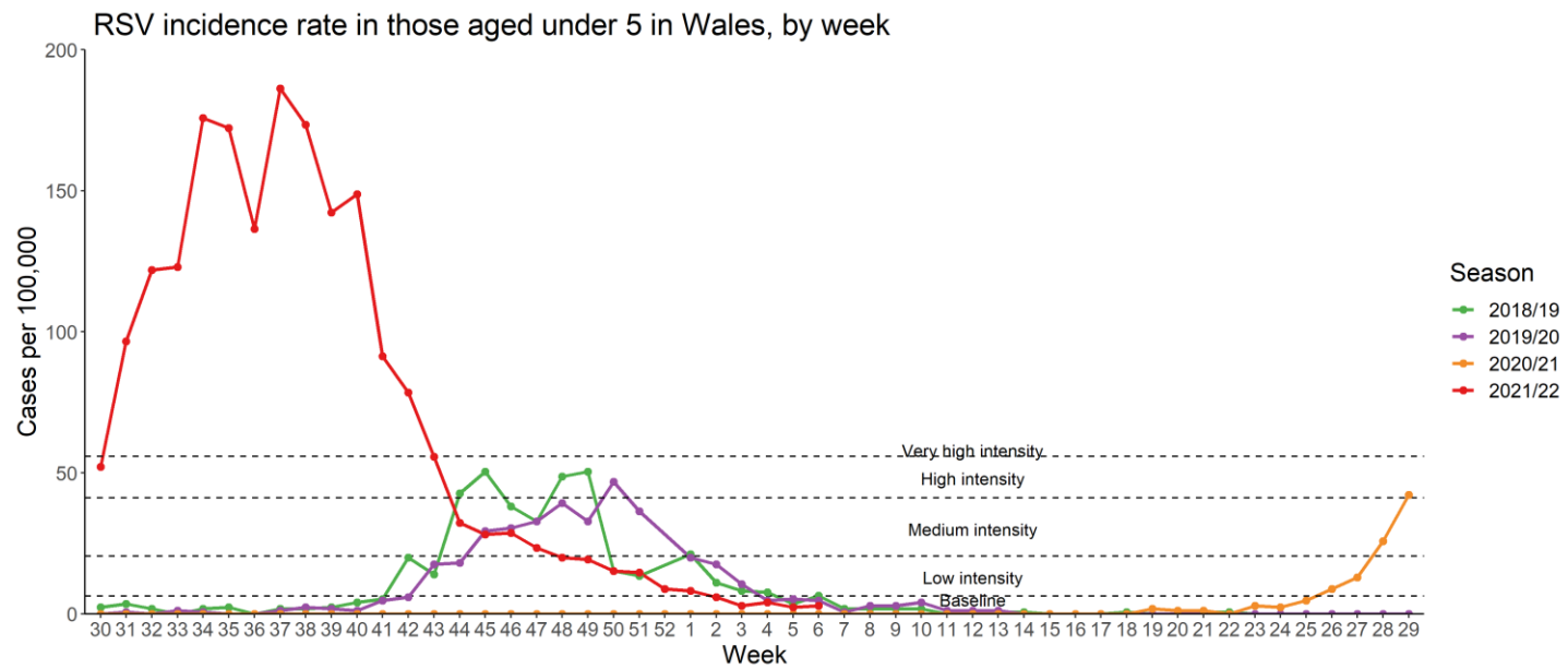
Figure 7. RSV incidence rate per 100,000 population aged under five years, week 30 2017 to Week 06 2022.
