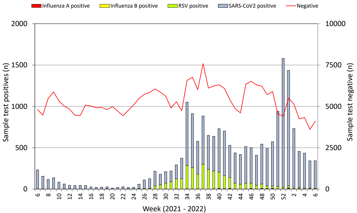
Figure 5. Specimens from hospital patients submitted for RSV, Influenza and SARS-CoV2 testing only, as of 13/02/2022 by week of sample collection, week 06 2021 to week 06 2022.
