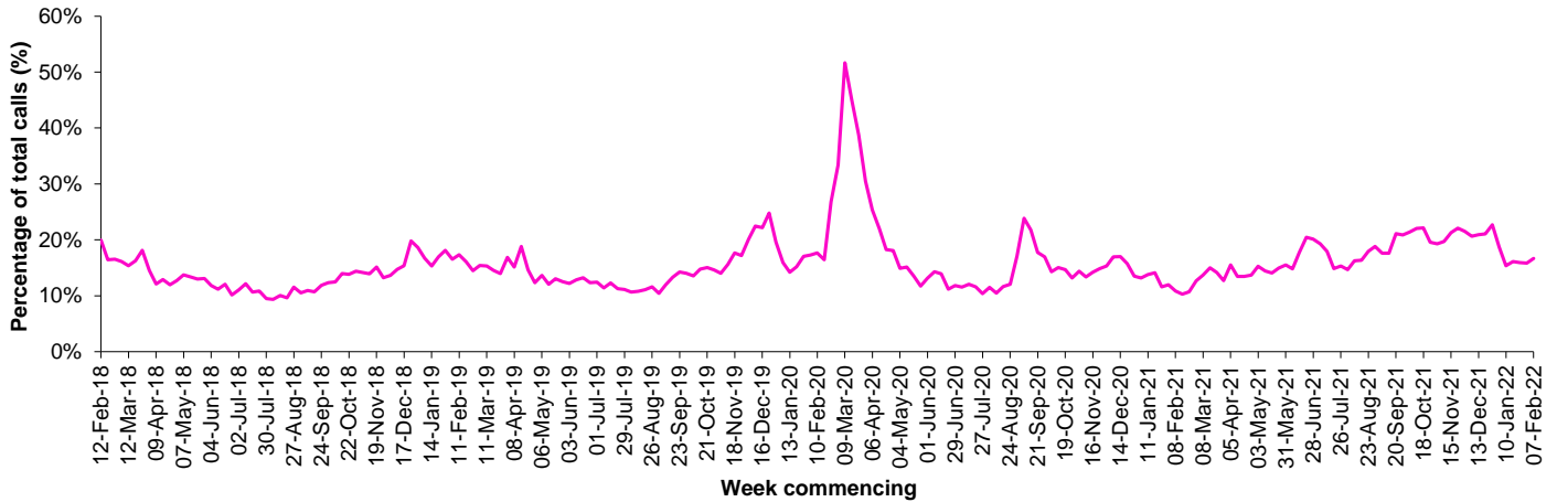
Figure 8. Influenza related calls to NHS Direct Wales 1 (as a percentage of total calls) from week 07 2018 - Week 06 2022 (as of 13/02/2022).
