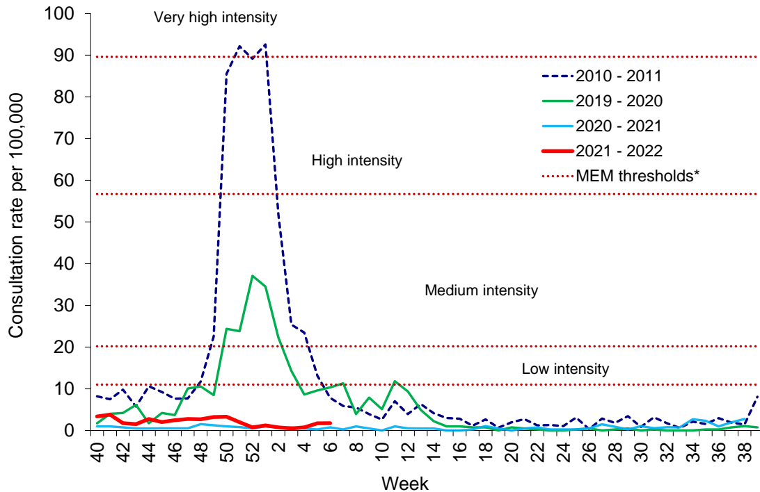
Figure 1. Clinical consultation rate for ILI per 100,000 practice population in Welsh sentinel practices (as of 13/02/2022).
