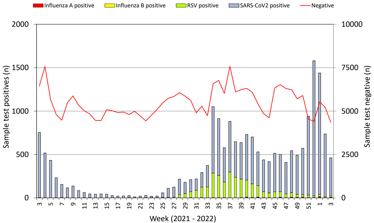
Figure 5. Specimens from hospital patients submitted for RSV, Influenza and SARS-CoV2 testing only, as of 23/01/2022 by week of sample collection, week 03 2021 to Week 03 2022.
