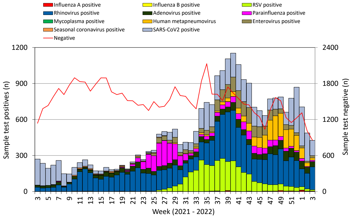
Figure 4. Specimens submitted for virological testing for hospital patients and non-sentinel GPs as of 23/01/2022 by week of sample collection, week 03 2021 to Week 03 2022.
