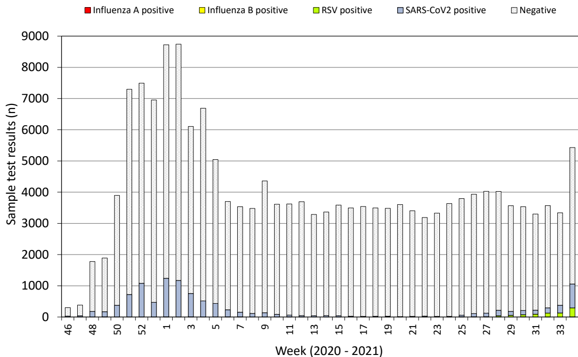
Figure 5. Specimens from hospital patients submitted for RSV, Influenza and SARS-CoV2 testing only, as of 29/08/2021 by week of sample collection, week 46 2020 to Week 34 2021.
