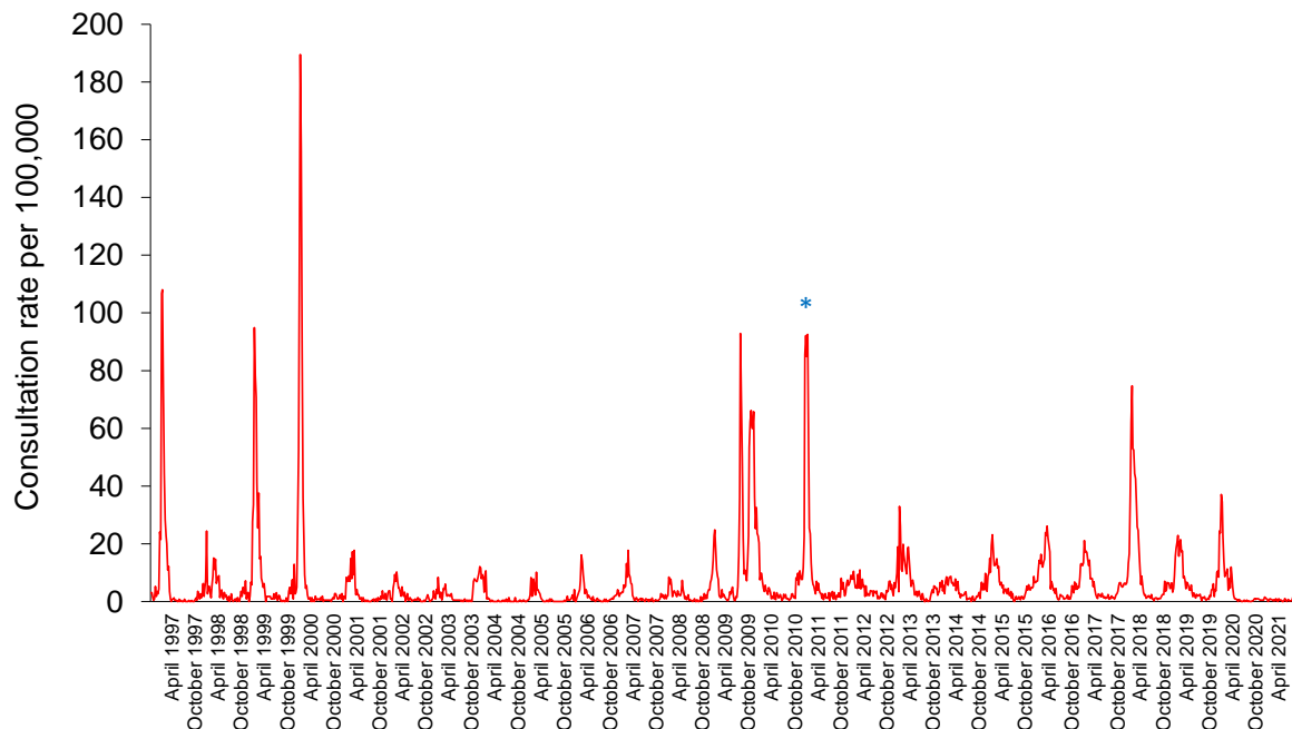
Figure 2. Clinical consultation rate for ILI per 100,000 practice population in Welsh sentinel practices (week 48 1996 – Week 34 2021).
