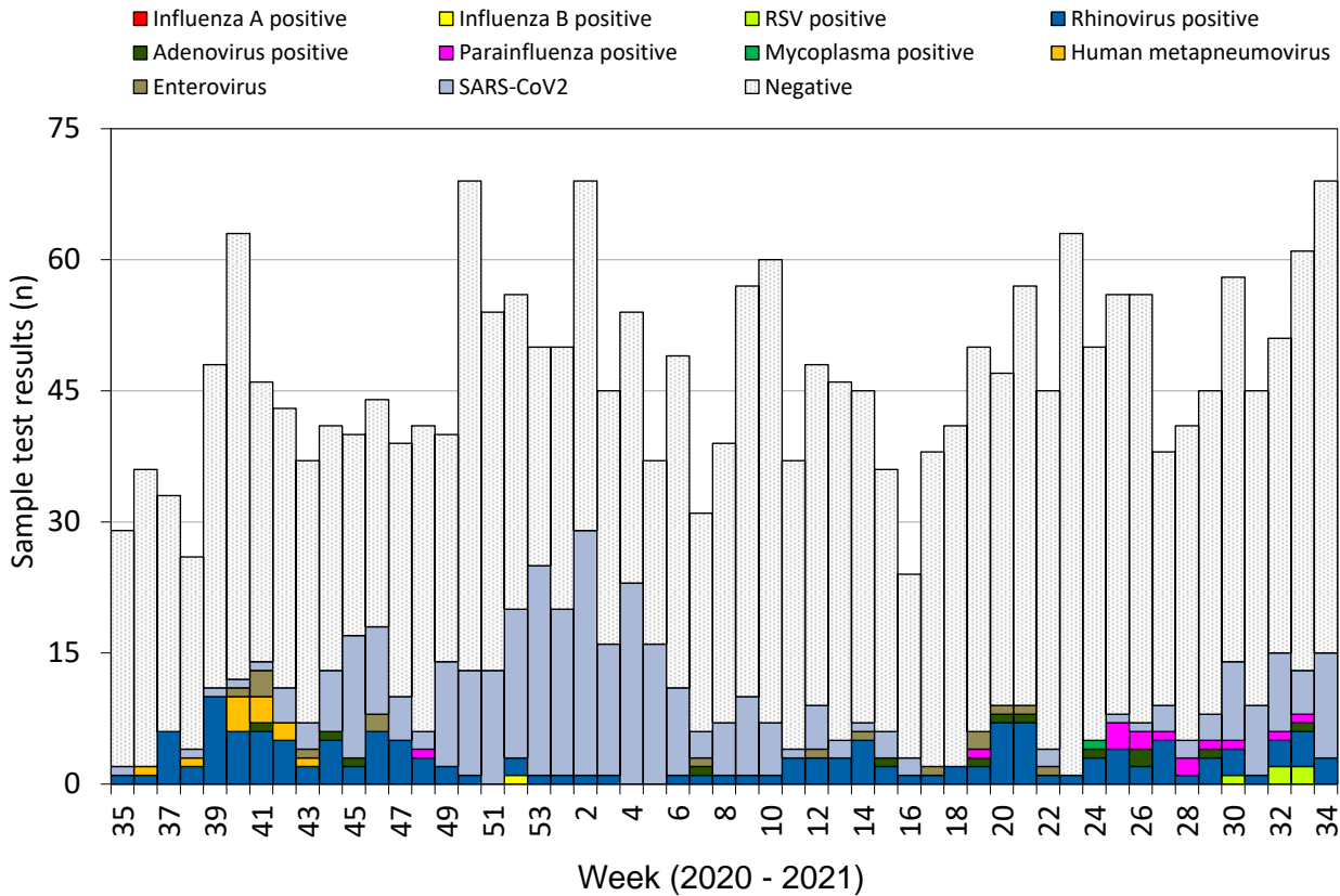
Figure 6. Specimens submitted for virological testing for ICU patients, by week of sample collection, week 35 2020 to Week 34 2021.
