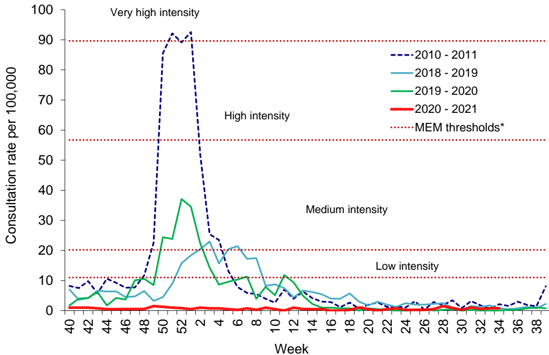
Figure 1. Clinical consultation rate for ILI per 100,000 practice population in Welsh sentinel practices (as of 29/08/2021).
