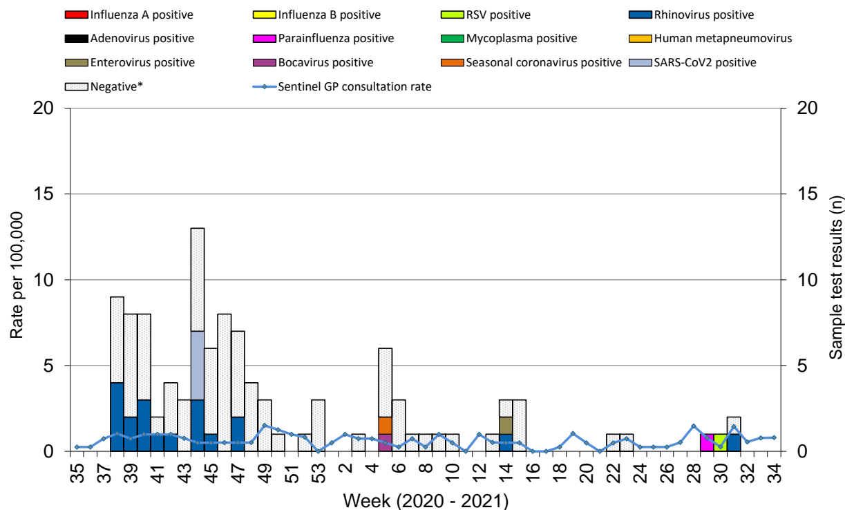
Figure 3. Specimens submitted for virological testing by sentinel GPs as of 29/08/2021, by week of sample collection, week 35 2020 to Week 34 2021.
