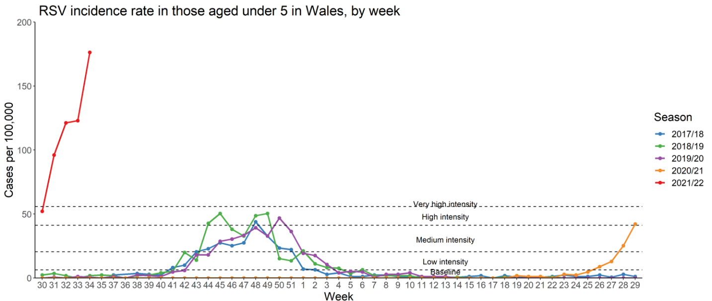
Figure 7. RSV incidence rate per 100,000 population aged under five years, week 30 2017 to Week 34 2021.
