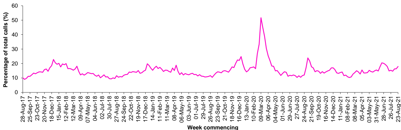
Figure 8. Influenza related calls to NHS Direct Wales 1 (as a percentage of total calls) from week 34 2017 - Week 34 2021 (as of 29/08/2021).
