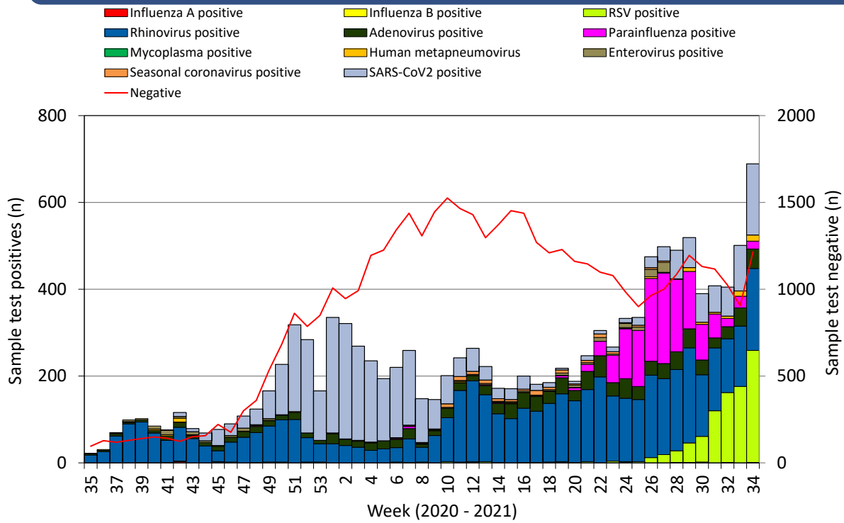
Figure 4. Specimens submitted for virological testing for hospital patients and non-sentinel GPs as of 29/08/2021 by week of sample collection, week 35 2020 to Week 34 2021.
